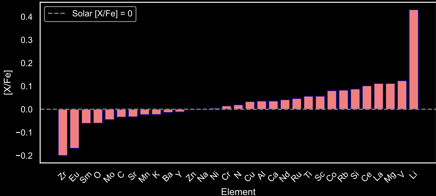
Abundance Pattern for GALAH Main Sequence Stars: Star Field [50] (N=139)
