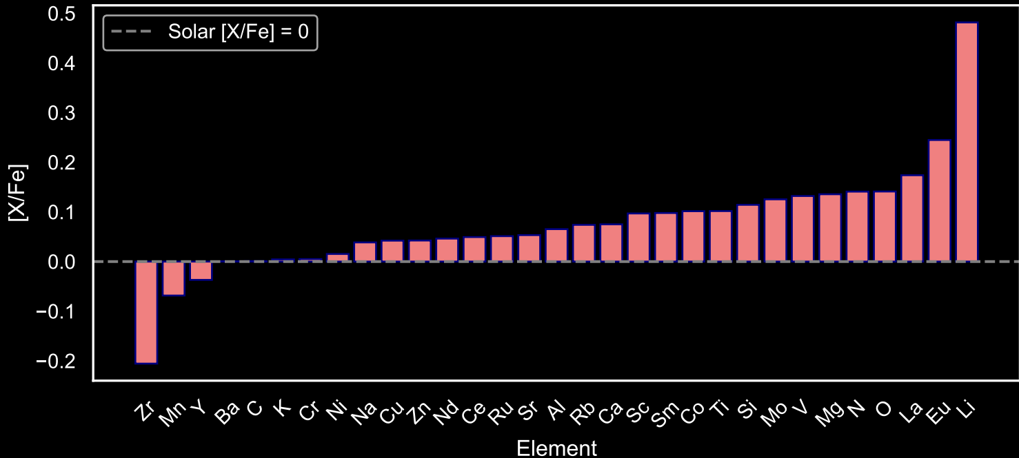
Abundance Pattern for GALAH Star Field [50] (N=296)
