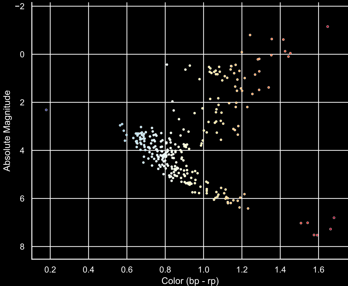
GALAH Hertzsprung-Russell Diagram Field [50] Ra [321.77] Dec [-52.4]
