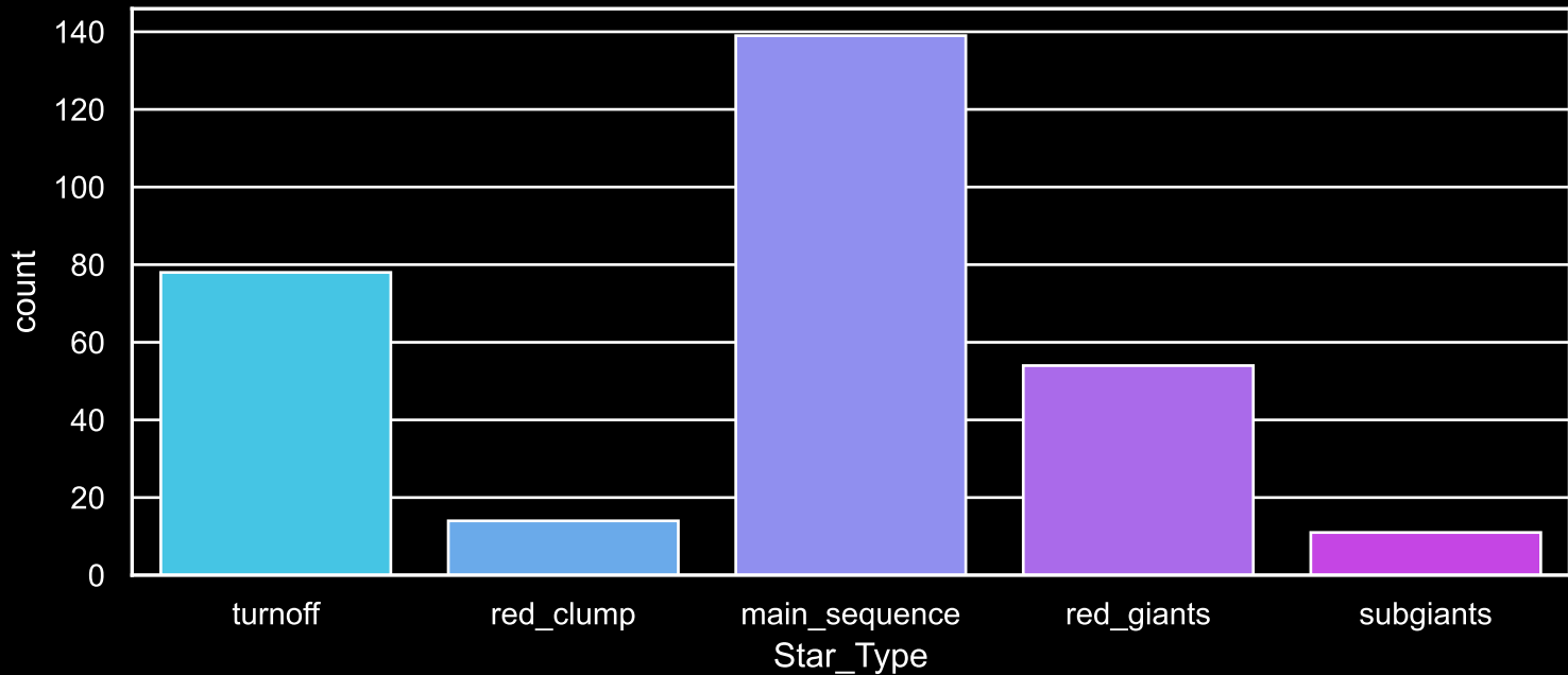
Field [50] Count plot of Star Type
