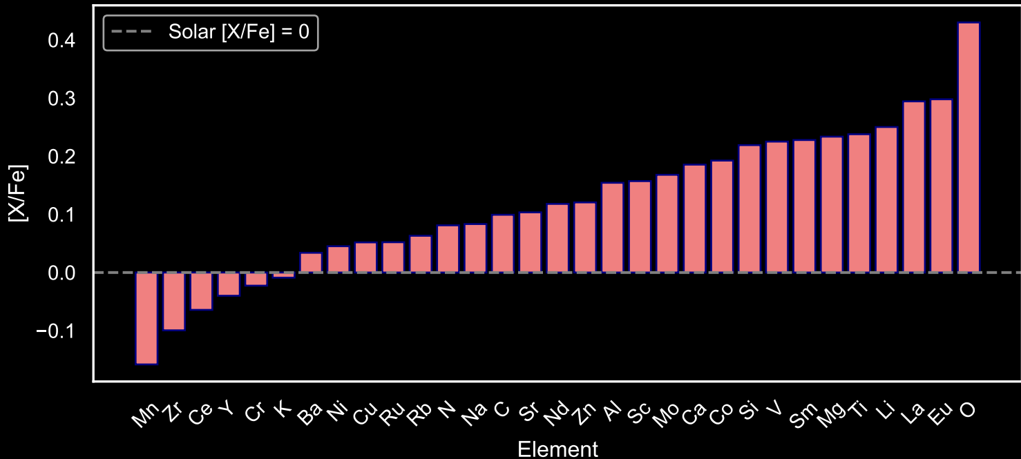
Abundance Pattern for GALAH Red Giants: Star Field [50] (N=68)
